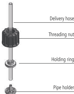
Fig 8. Delivery hose / pump head assembling
